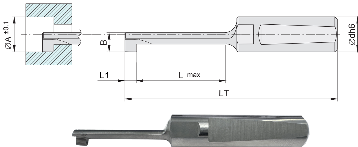
ATTACCO WHISTLE NOTCH - Whistle Notch Shank
